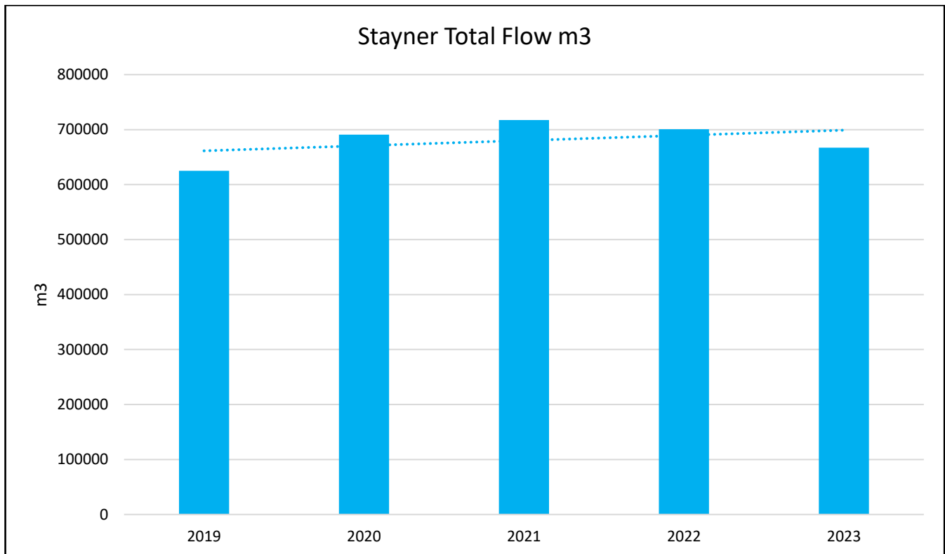
Figure 4: Five-year Total Flow Comparison
