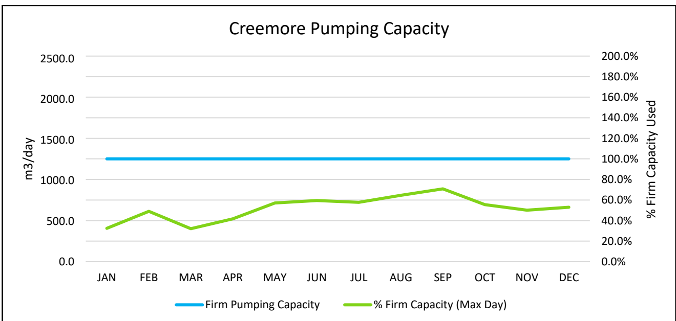
Figure 2: System Capacity
