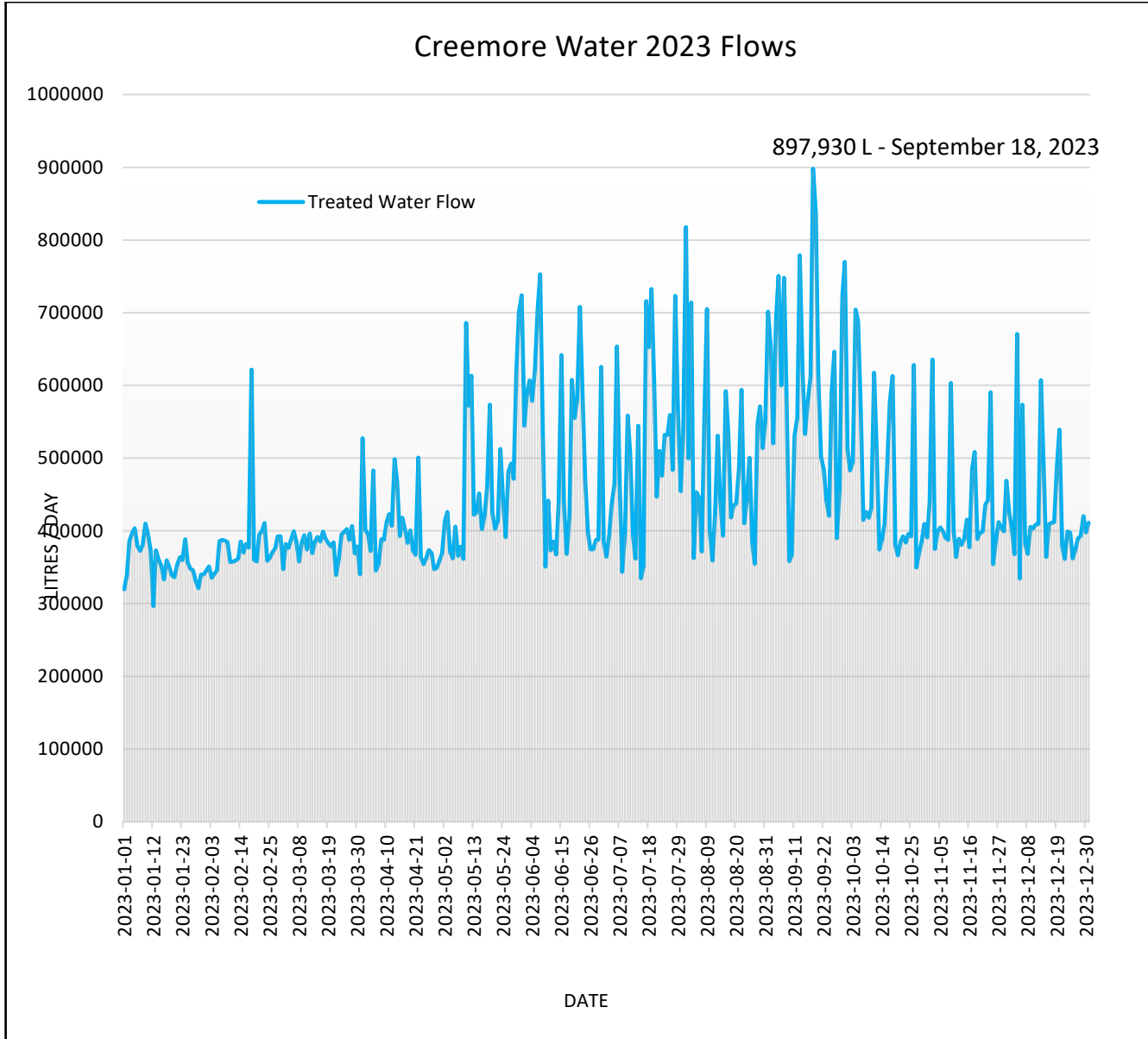
Figure 3: 2023 Daily Flows
