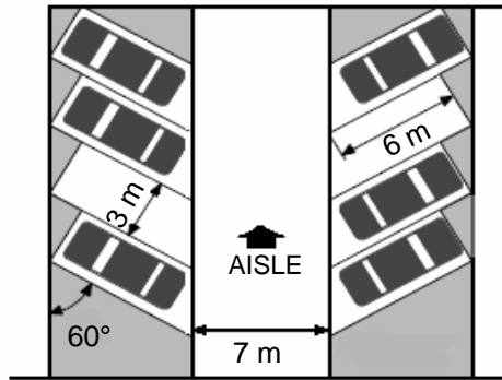
ANGLED PARKING
