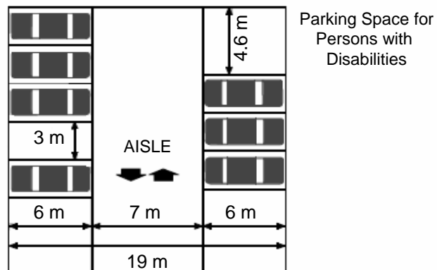
TYPICAL PARKING
