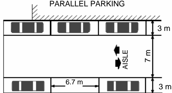
TYPICAL PARKING
